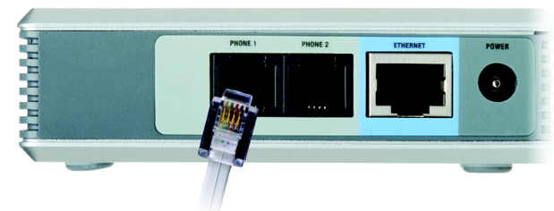
Figure 3-2: Connect the RJ-11 Telephone Cable
